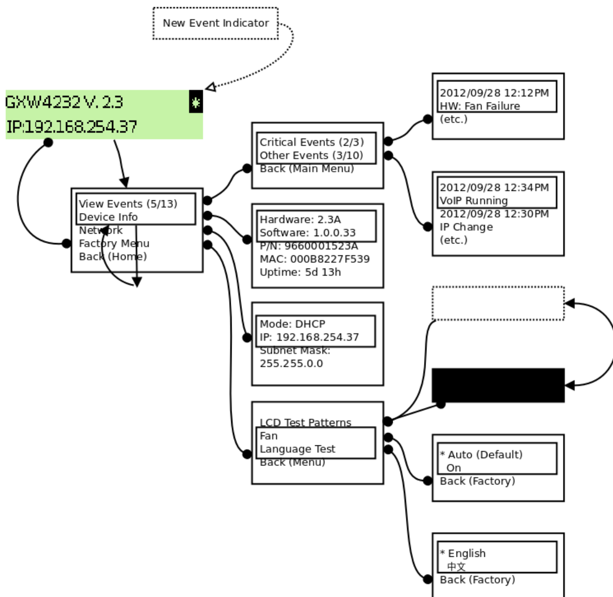
FIGURE 3: LCD MENU
