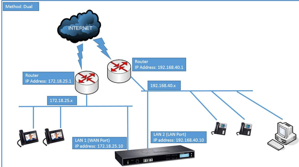
Figure 9: UCM6510 Network Interface Method: Dual
