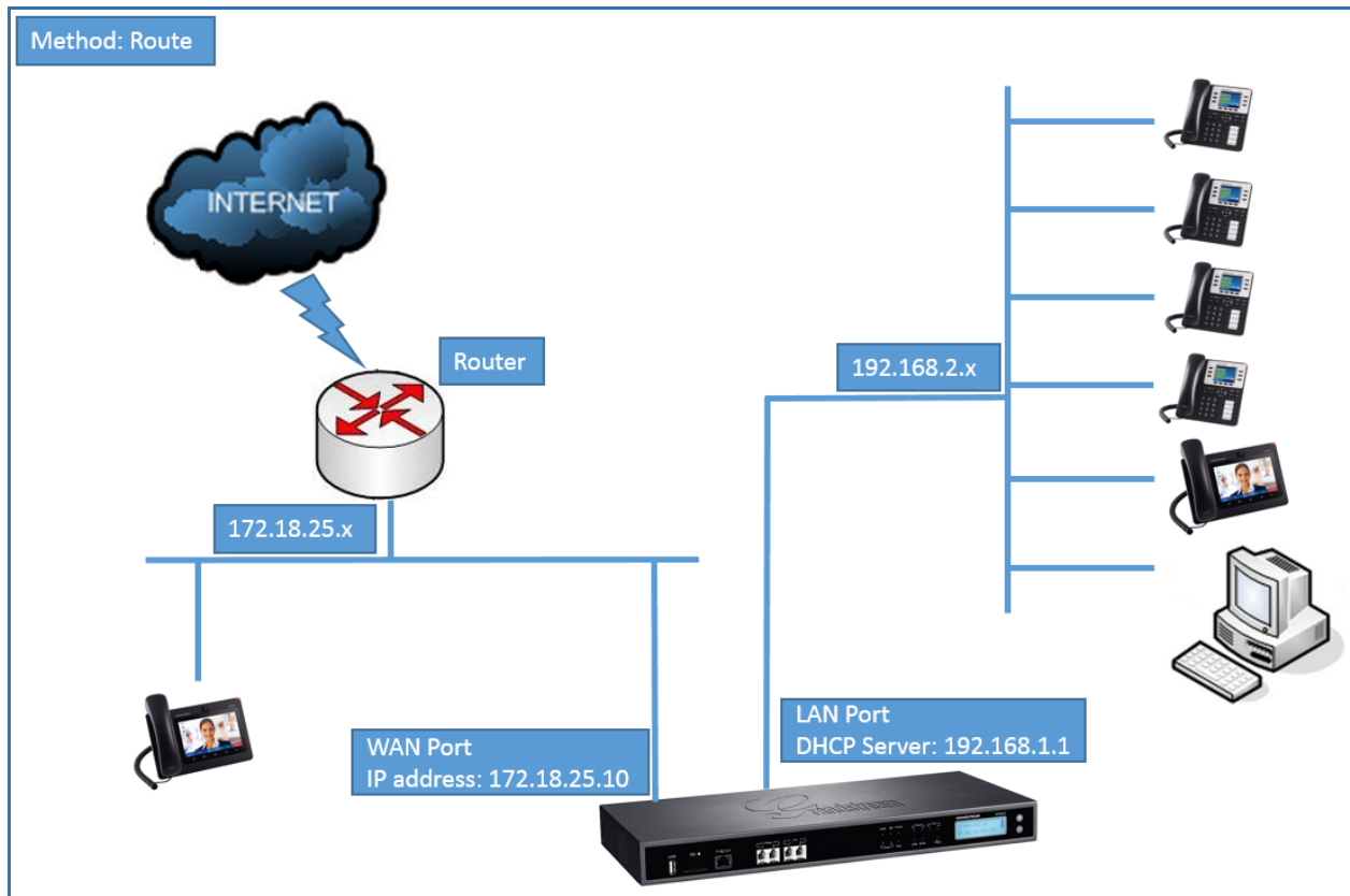
Figure 7: UCM6510 Network Interface Method: Route
