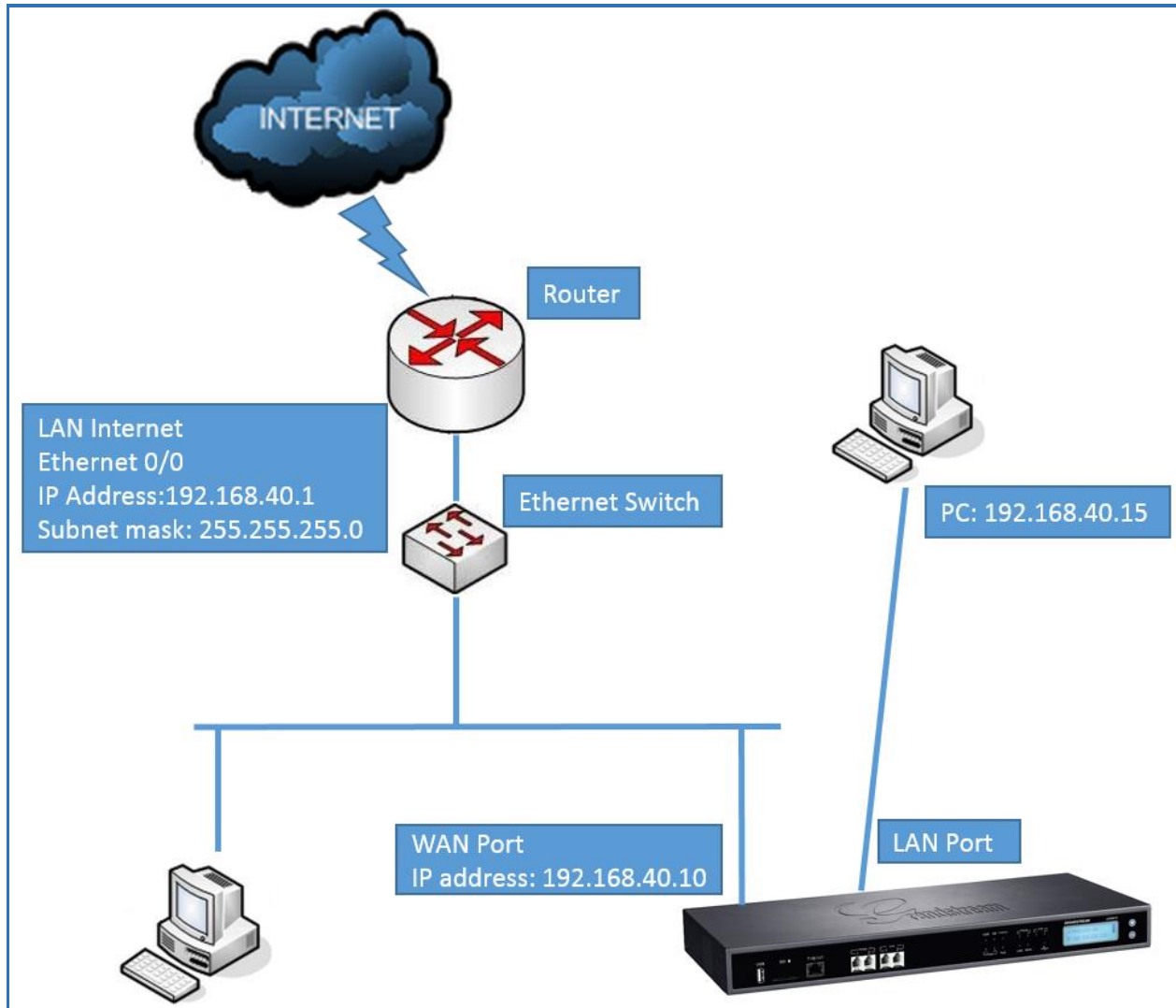
Figure 8: UCM6510 Network Interface Method: Switch
